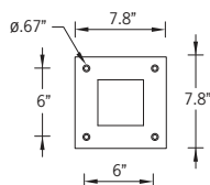
Mounting Detail
