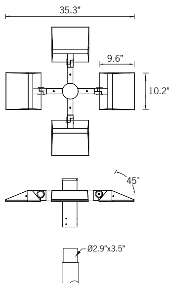
Tenon Detail
