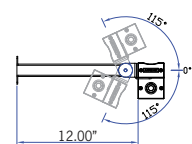
ADJ12 - 12' Extended Arm
