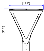
Fixture Detail
