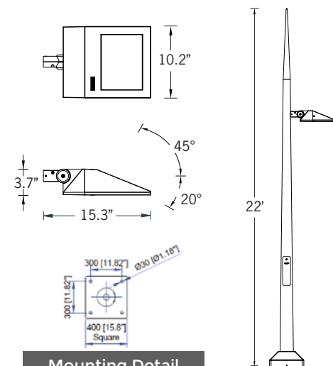
Mounting Detail
