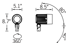
Floodlight Detail
