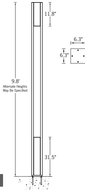
Mounting Detail
