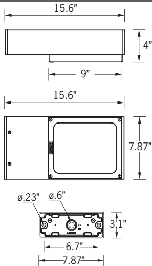
Mounting Detail
