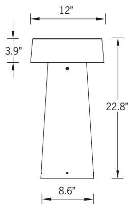
Mounting Detail
