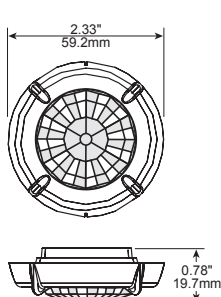
FSP-L3 dimensions
