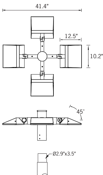
Tenon Detail
