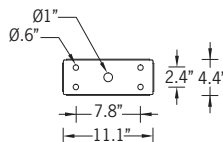
Mounting Detail
