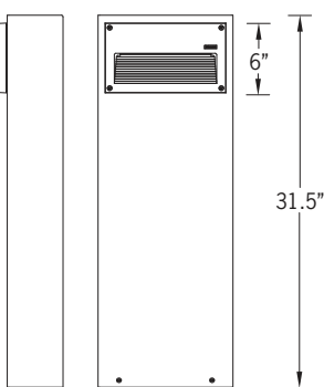
Mounting Detail
