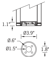
Mounting Detail
