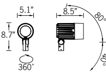
Floodlight Detail
