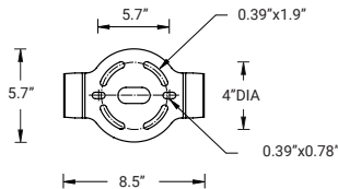
Mounting Detail
