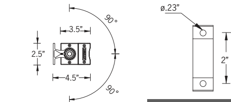
Mounting Detail
