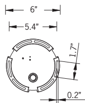
Mounting Detail
