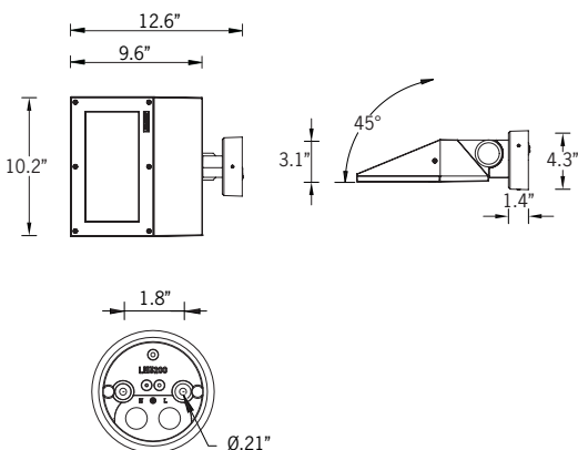
Mounting Detail
