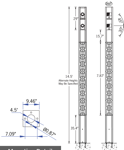
Mounting Detail
