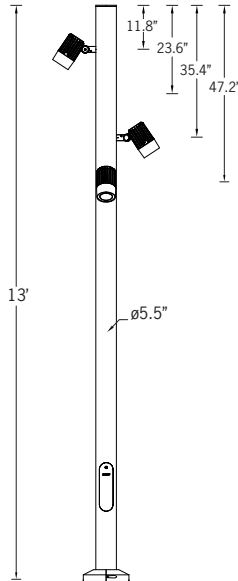
Floodlight Detail
