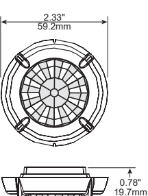
FSP-L3 dimensions
