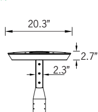
Fixture Detail
