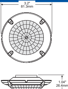
FSP-L7 dimensions
