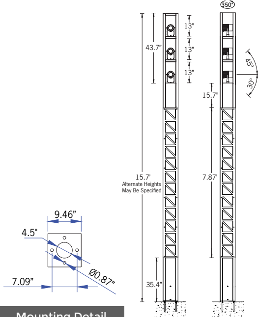
Mounting Detail
