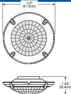
FSP-L7 dimensions
