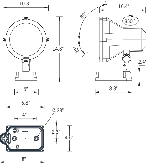
Mounting Detail
