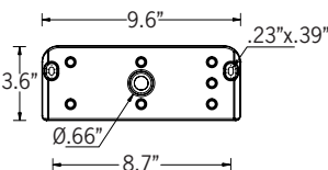
Mounting Detail
