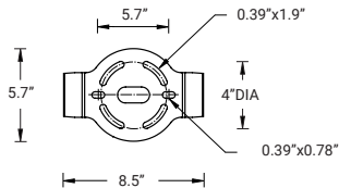
Mounting Detail
