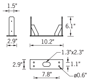
Mounting Detail
