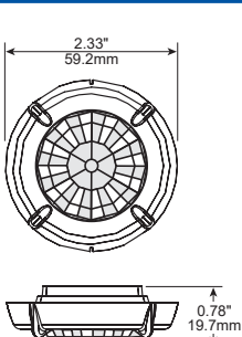
FSP-L3 dimensions
