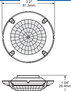
FSP-L7 dimensions
