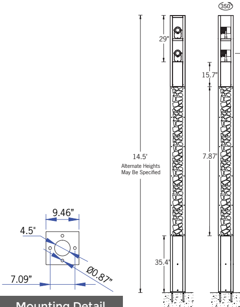
Mounting Detail
