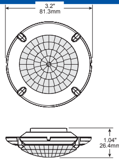
FSP-L7 dimensions
