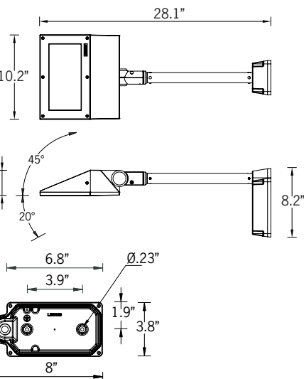
Mounting Detail
