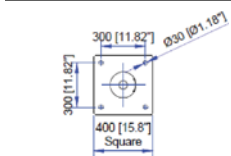
Mounting Detail
