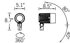
Floodlight Detail
