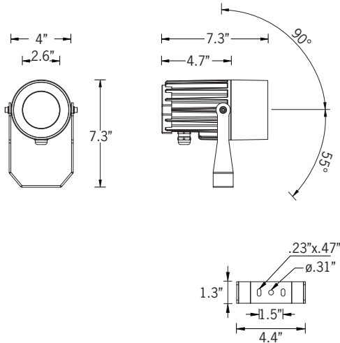
Mounting Detail
