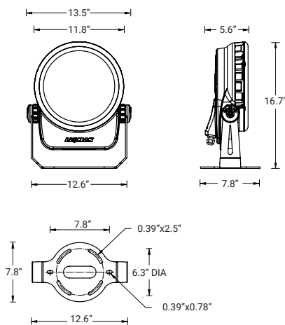
Mounting Detail
