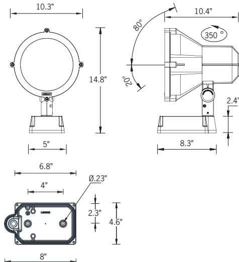
Mounting Detail
