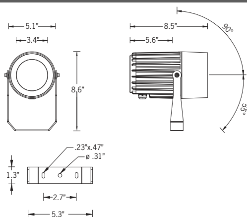
Mounting Detail
