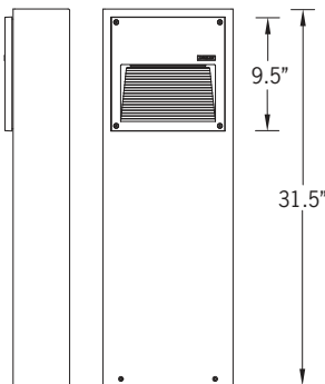
Mounting Detail
