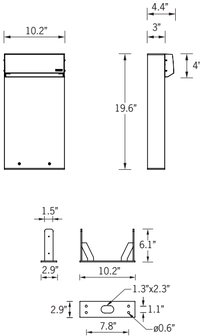
Mounting Detail
