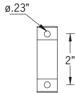
Mounting Detail
