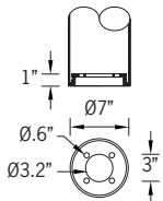
Mounting Detail
