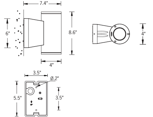
Mounting Detail
