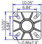
Mounting Detail
