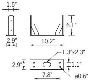
Mounting Detail
